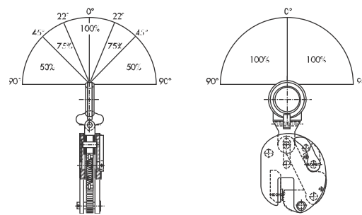
Plate lifting clamps type EU and EUS. Load reduction should be applied as per load direction angle and corresponding remaining percentage of the Working Load Limit.
